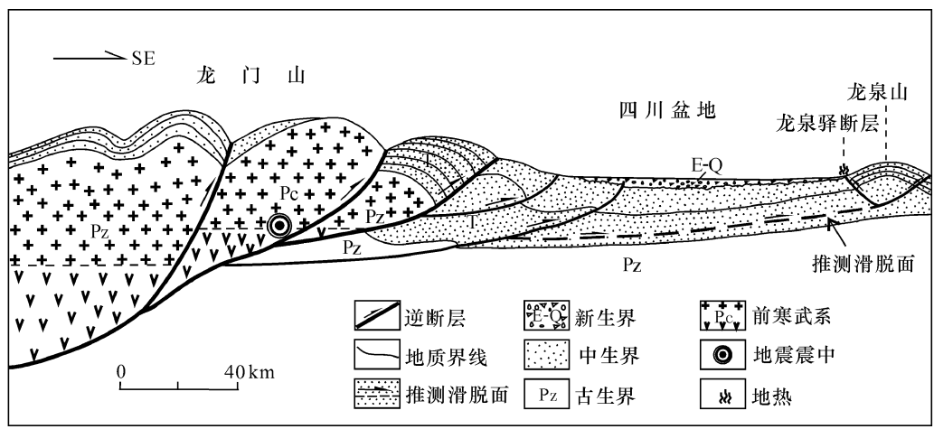
图 3 龙门山推覆构造带及龙泉山背斜构造示意剖面图 Fig.3 Cross section through the nappy structural belts of the Longmenshan to the Longquanshan anticline
