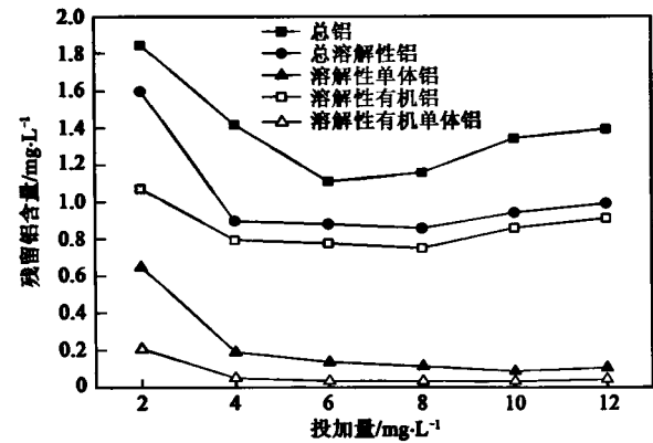
图6 氯化铝混凝沉淀出水中不同组分残留铝的含量 Fig.6 Content of different residual aluminum speciation in the effluent after coagulation and sedimentation with AlCl 3
