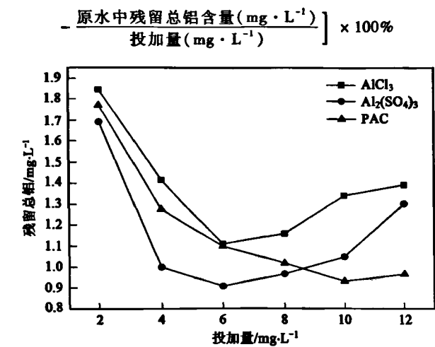
图5 3种混凝剂混凝出水中残留总铝含量 Fig.5 Residual aluminum content of three Al-based coagulants in the effluent
