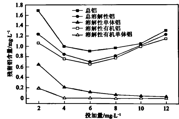
图7 硫酸铝混凝沉淀出水中不同组分残留铝的含量 Fig.7 Content of different residual aluminum speciation in the effluent after coagulation and sedimentation with Al 2 (SO 4 ) 3
