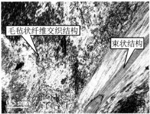
图 1 角闪石的毛毡状纤维交织结构和束状结构 Fig. 1 Felted fibrous interlocking and sheaflike textures of hornblende
